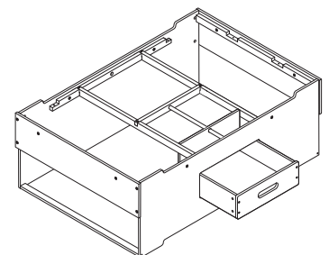
Assembled View
