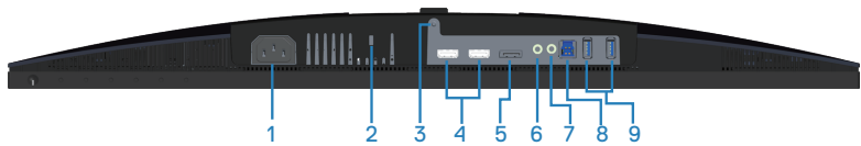
Bottom view without monitor stand (S2419HGF)
