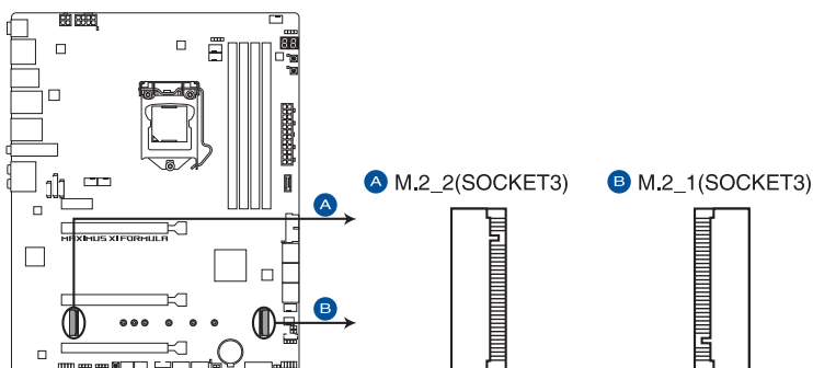
ROG MAXIMUS XI FORMULA M.2(SOCKET3)
