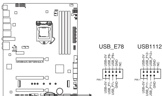
ROG MAXIMUS XI FORMULA USB 2.0 connectors
