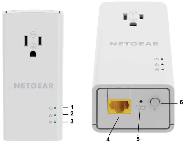
Figure 7. Hardware features
