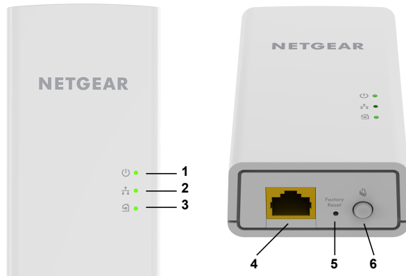
Figure 1. Hardware features
