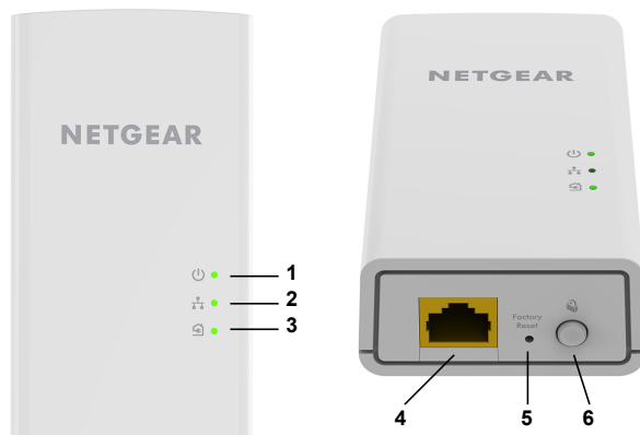
Figure 6. Hardware features
