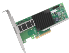
Brand Name Intel® Ethernet Converged Network Adapter XL710-QDA1
