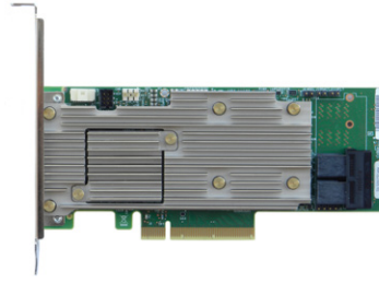
INTEL® RAID CONTROLLER RSP3DD080F
